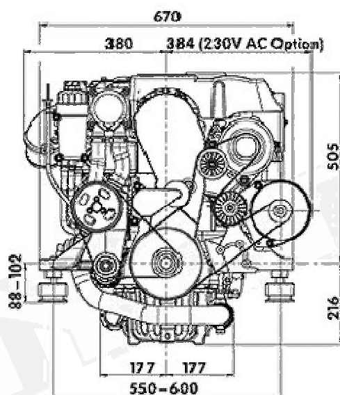
Frontal view
